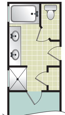
MASTER BATH WITH GARDEN TUB
